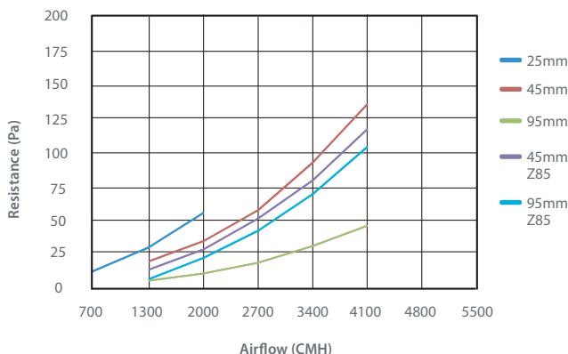
Aero Carb Z - Airflow vs. Initial Resistance
